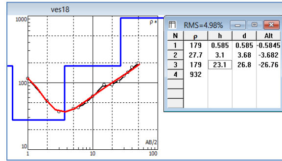
Figure 3d: Curve Type HA.
