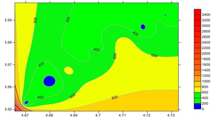
Figure 4d: Contour Resistivity Layer 4.
