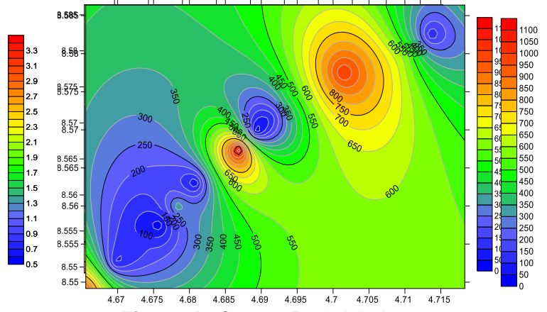
Figure 4b: Contour Resistivity Layer 2.
