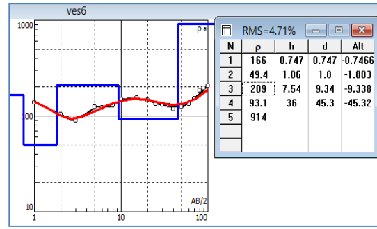
Figure 3b: Curve Type HKH.
