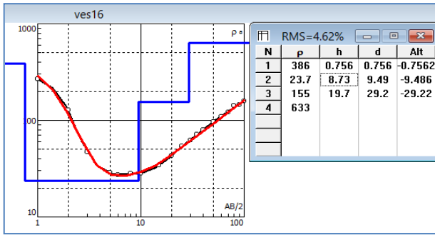
Figure 3a: Curve Type H.
