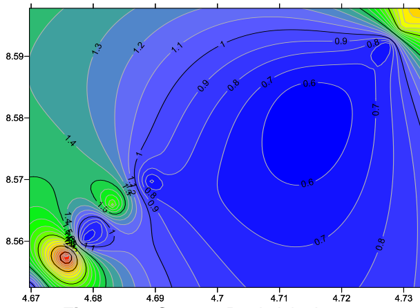
Figure 4a: Contour Resistivity Layer 1.
