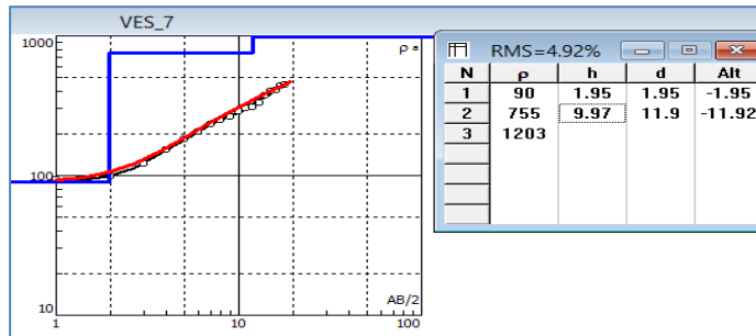
Figure 3e: Curve Type A.
