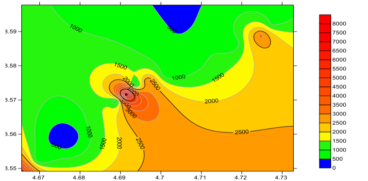
Figure 4e: Contour Resistivity Layer 5.
