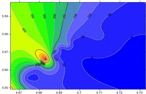
Figure 4c: Contour Resistivity Layer 3.
